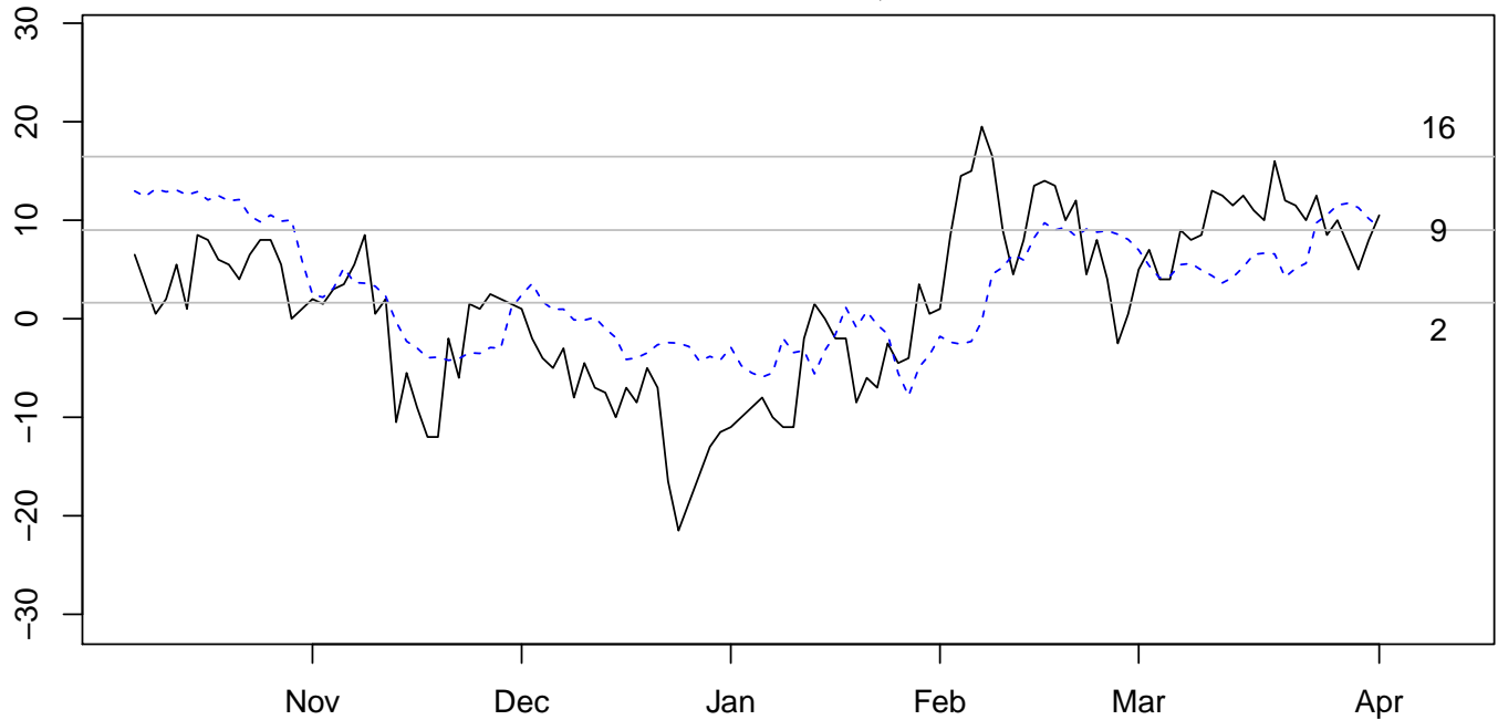
Actual minus Modelled. Last Value = $1 (0.27SD)
