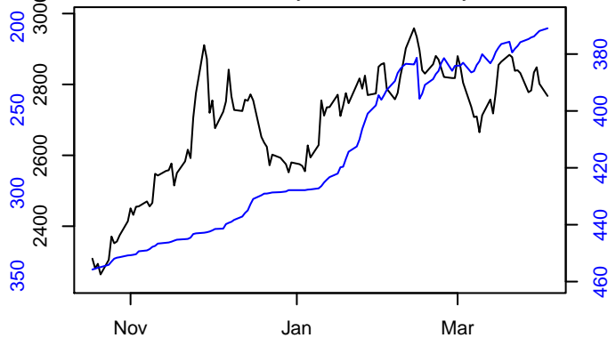
Pb3M and LME Lead Stock. correlations 120 day: -0.26 , 60 day: -0.16
