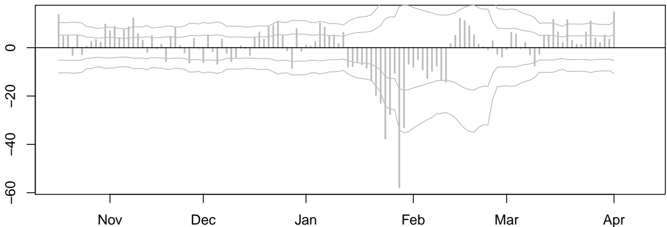
Standard Deviation (SD) Lines (-2, -1, 1, 2): grey.
