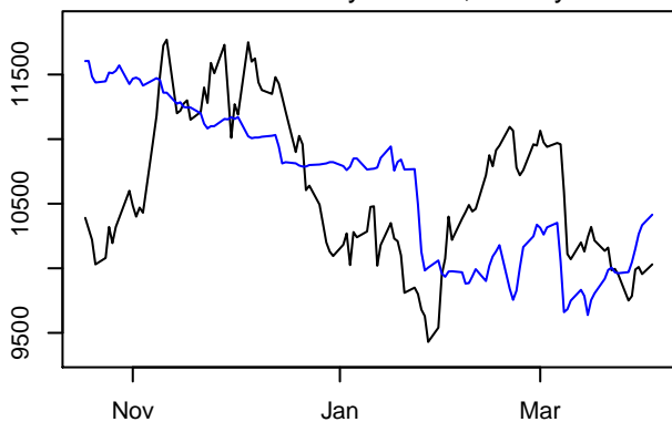
Ni3M and LME Nickel Stock. correlations 120 day: -0.38 , 60 day: 0.08
