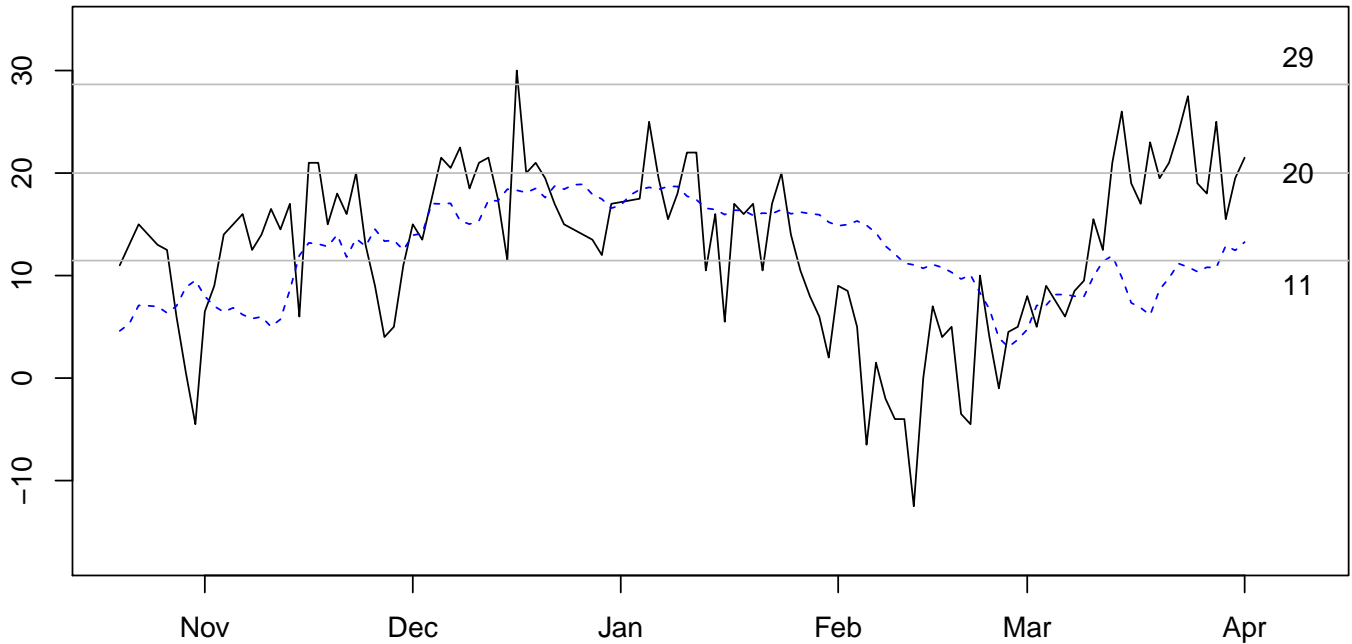
Actual minus Modelled. Last Value = $8 (1.46SD)
