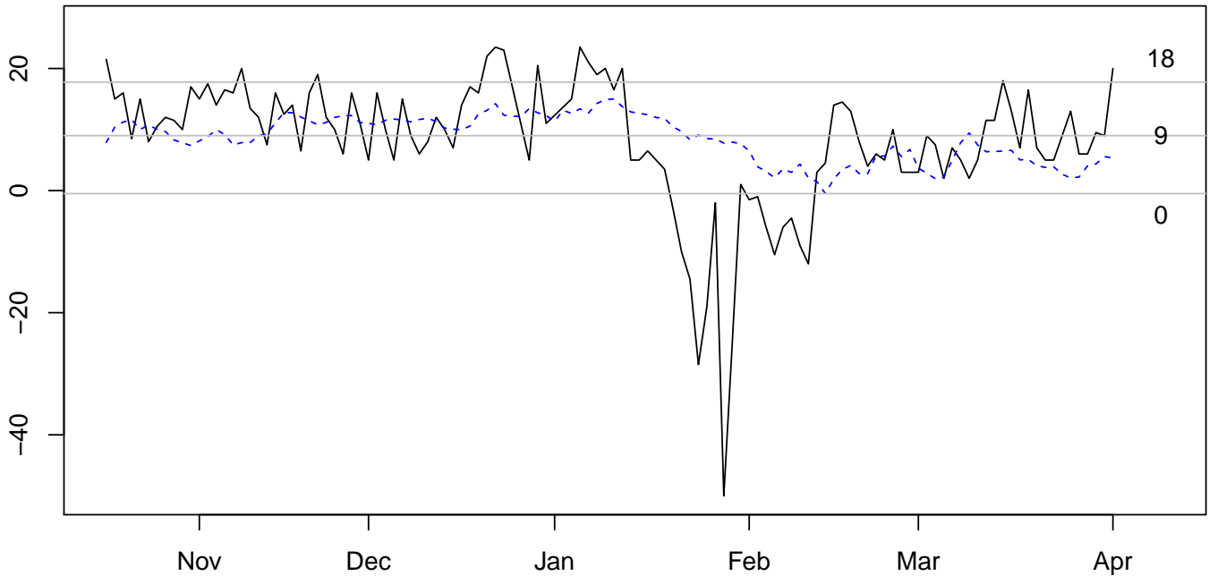
Actual minus Modelled. Last Value = $15 (2.76SD)
