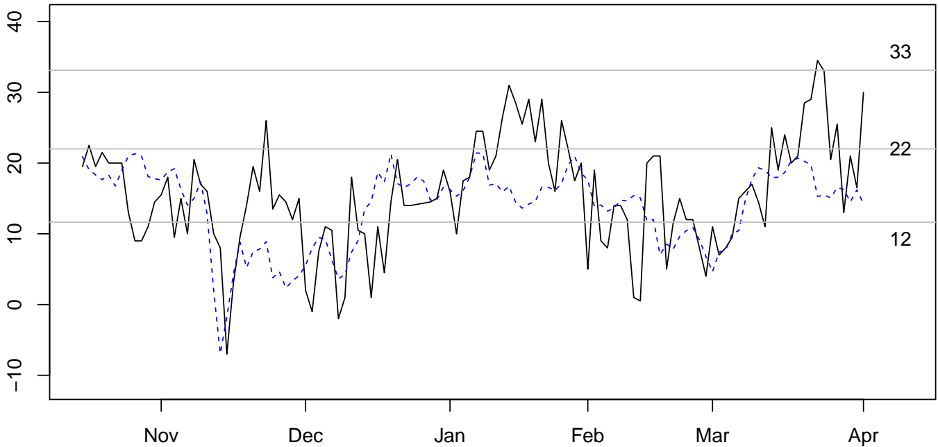
Cu Spread (actual: black line, modelled: blue dashed line). 03 Apr 2017 Last Values : Actual $30, Modelled $14.
