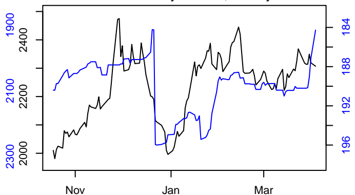
Sn3M and LME Tin Stock. correlations 120 day: -0.72 , 60 day: -0.63
