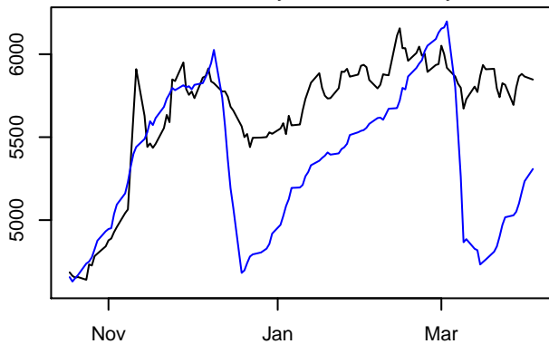
Al3M and LME Aluminium Stock. correlations 120 day: -0.27 , 60 day: -0.76
