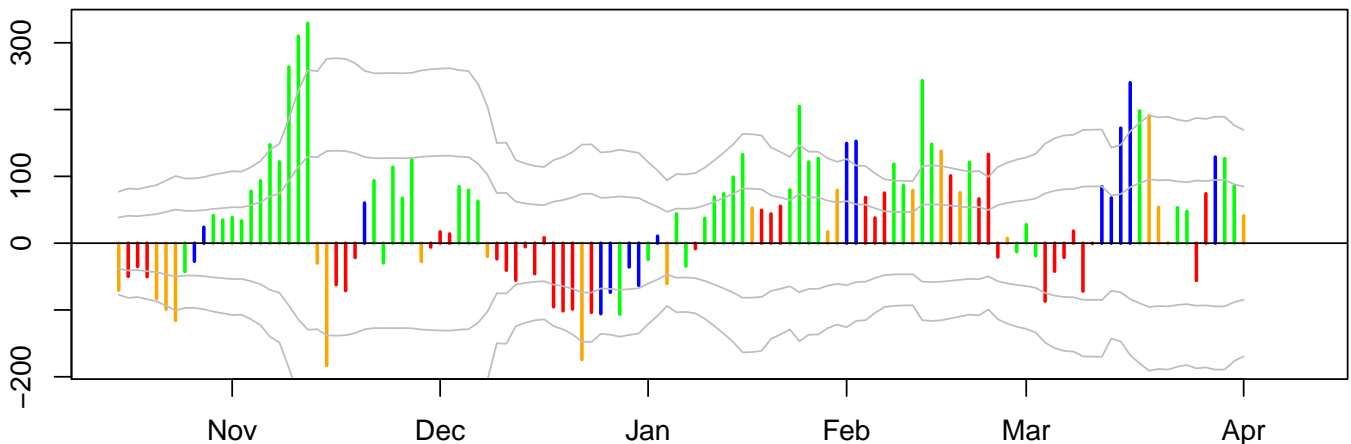
Bar Colour (Actual | Modelled Momentum) : red (-2), orange (-1), blue (1), green (2). Standard Deviation (SD) Lines (-2,-1, 1, 2): grey.
